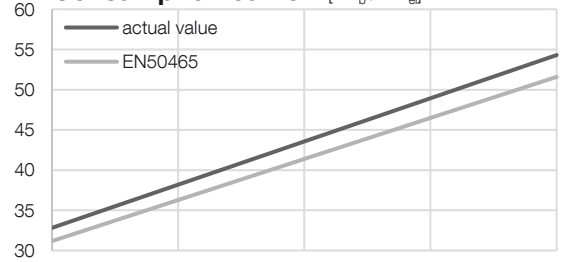
Consumption curve 3) [kW o / kW el ]
