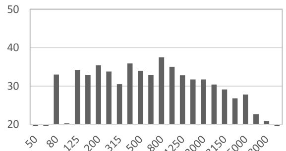
Sound pressure level curve 6) 9) [dB(A)/ Hz]
