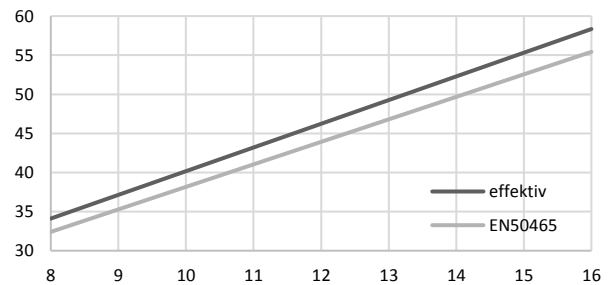
Consumption curve 3) [kW b / kW el ]
