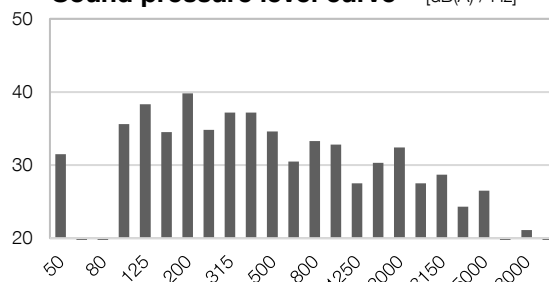
Sound pressure level curve 6) [dB(A) / Hz]
