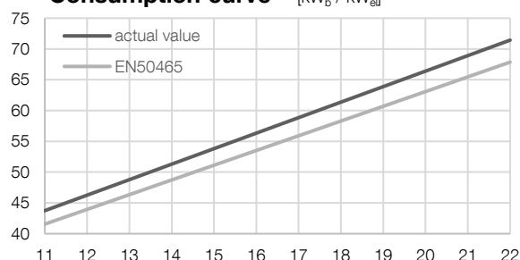
Consumption curve 3) [ kW_b / kW_{el} ]
