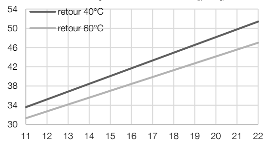
Courbes de performance [kW th /kW e ]
