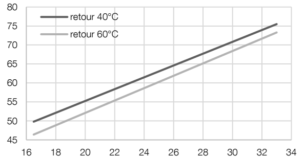
Courbes de performance [kWth / kWel]
